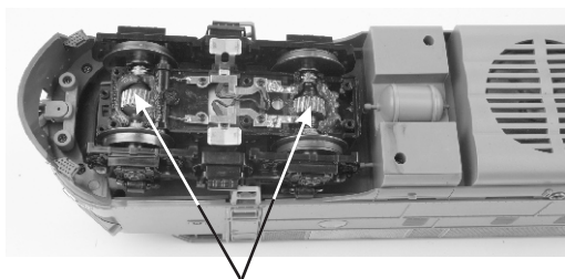
Figure 26: Grease Points Inside Power Truck
