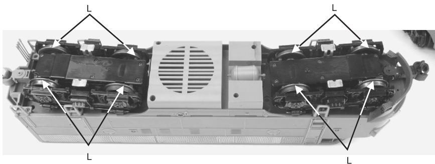
Figure 24: Lubrication Points on the Locomotive
