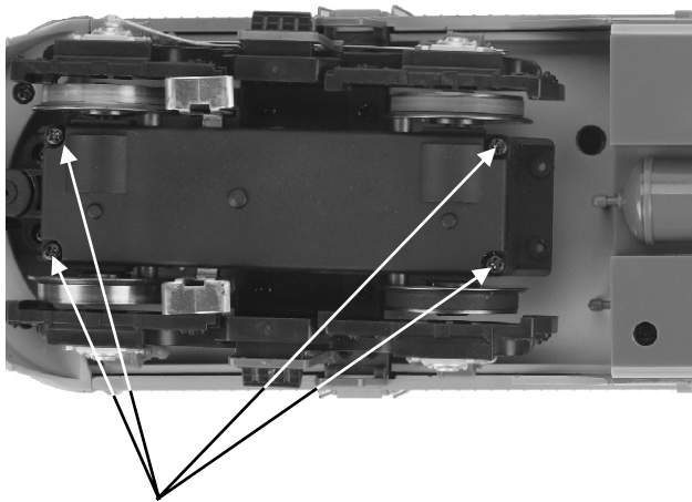
Figure 25: Truck Bottom Plate Mounting Screws
